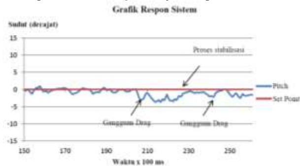
Gambar 12 Grafik respon Remotely Operated Vehicles (ROV) pada kondisi surge
