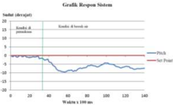
Gambar 10 Grafik respon kontrol open loop pada Remotely Operated Vehicles (ROV)
