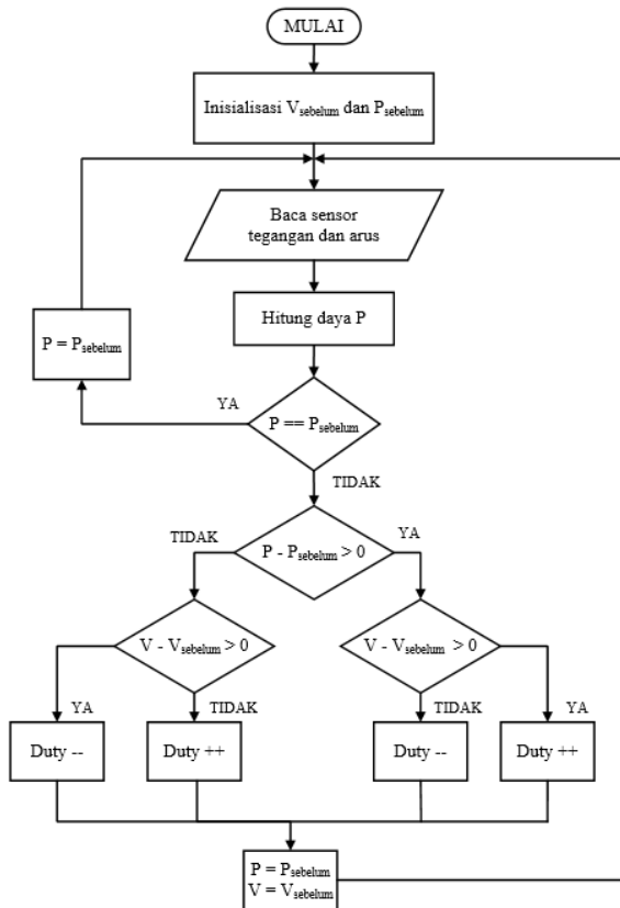
Gambar 5. Diagram alir metode Perturb and Observe
