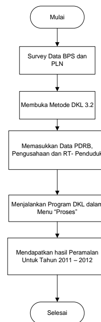
Gambar 2. Diagram Alir DKL 3.2
