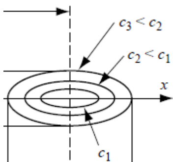
Gambar 9. Fenomena dispersi
