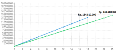
Perbandingan Crashing
