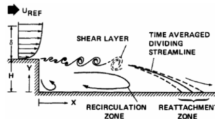
Gambar 3. Skema backward-facing step aliran turbulen [4].
