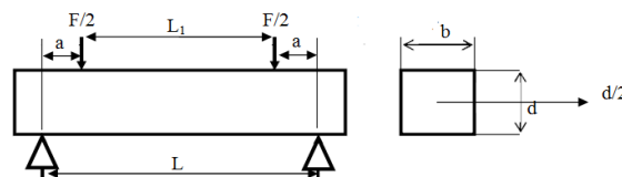
Gambar 6. Uji four point bending .
