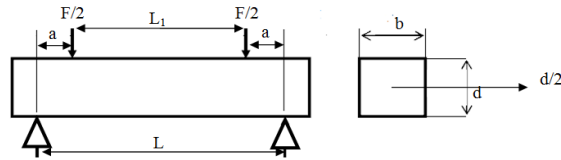
Gambar 2. Uji four point bending .
