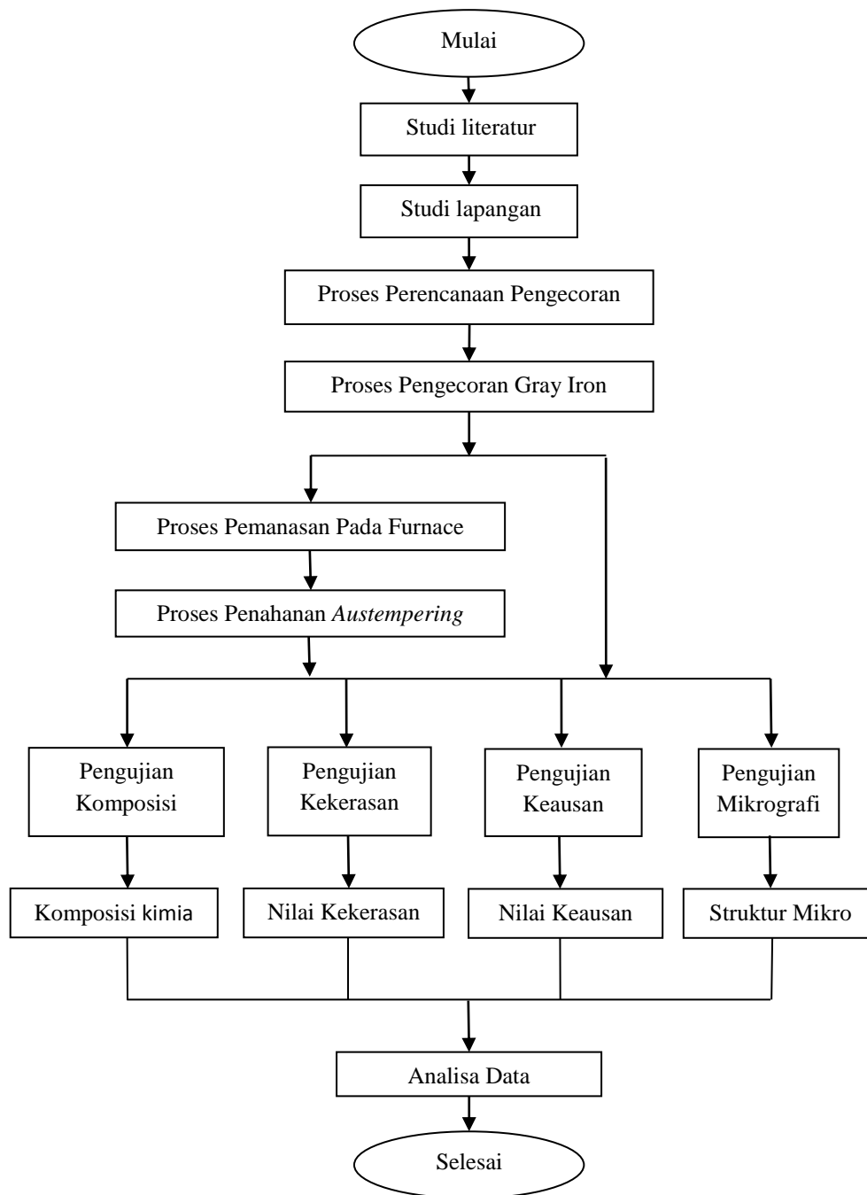
Gambar 1. Flowchart penelitian
