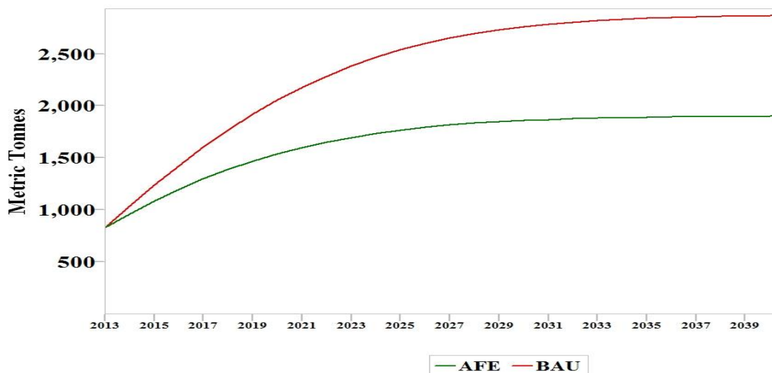
Gambar 5. Grafik Perbandingan Emisi Gas Buang Jenis Nitrogen Oxides (NO x ) pada Skenario Business as Usual dan Advanced Fuel Economy
