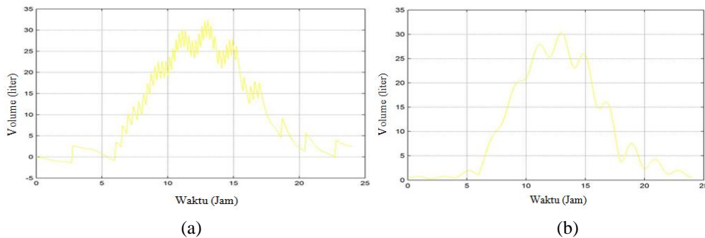
Gambar 12. (a) Volume air hasil kontroler on/off, (b) Volume air hasil kontroler PI
