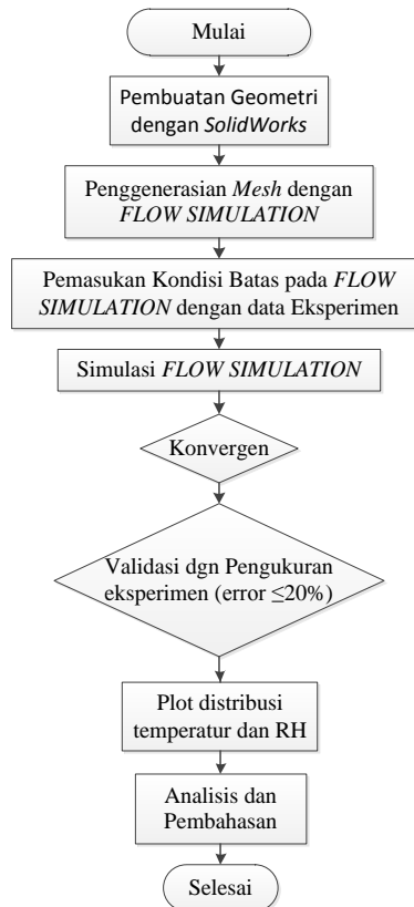
Gambar 3. Flowchart penelitian
