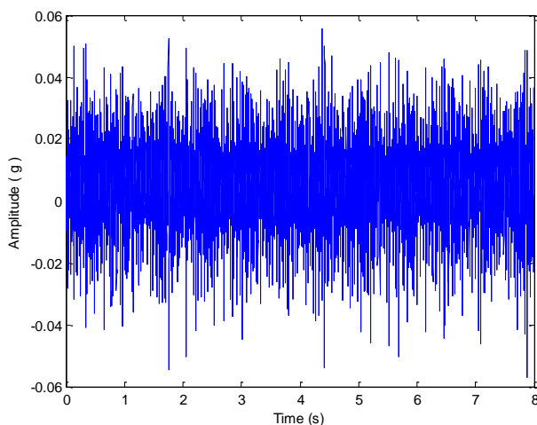
Gambar 5. Baseline 1000 rpm
