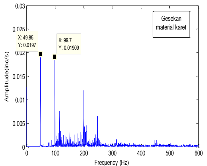
Gambar 18. Karet rub (3000 rpm)
