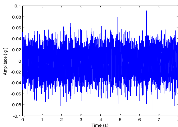
Gambar 7. Baseline (2000 rpm)
