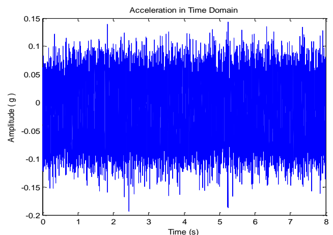
Gambar 8. Aluminium rub (2000 rpm)
