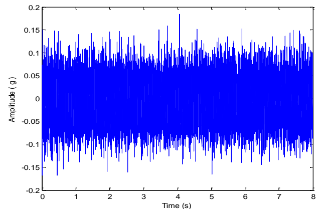
Gambar 10. Aluminium rub (3000 rpm)
