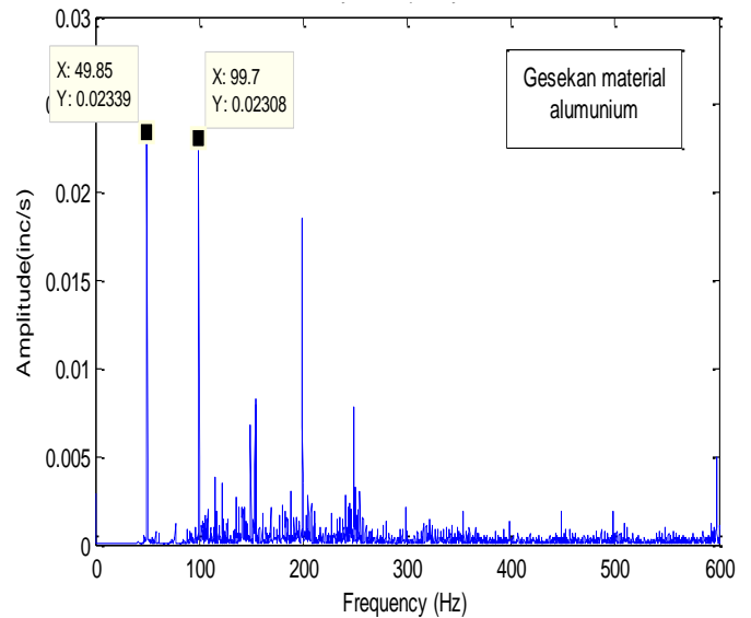
Gambar 16. Aluminium rub (3000 rpm)
