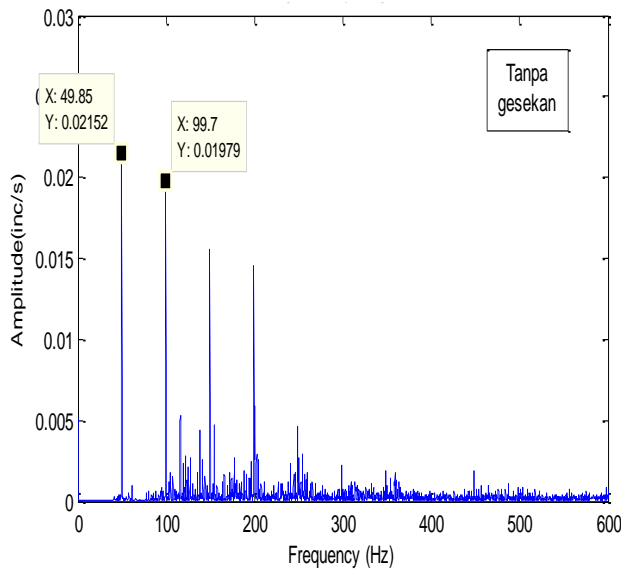
Gambar 15. Baseline (3000 rpm)
