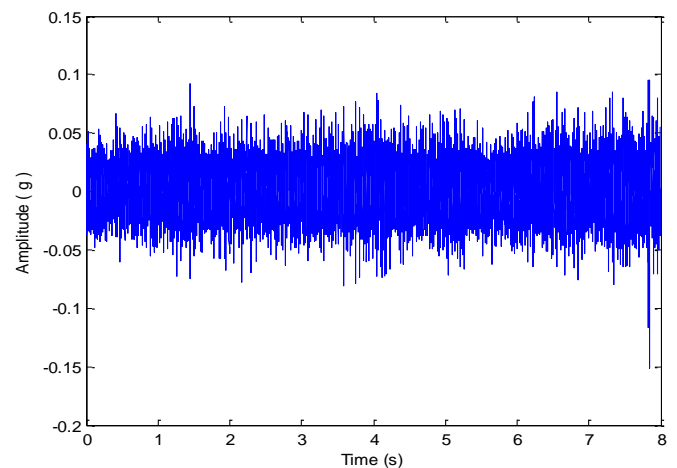
Gambar 6. Aluminium rub (1000 rpm)
