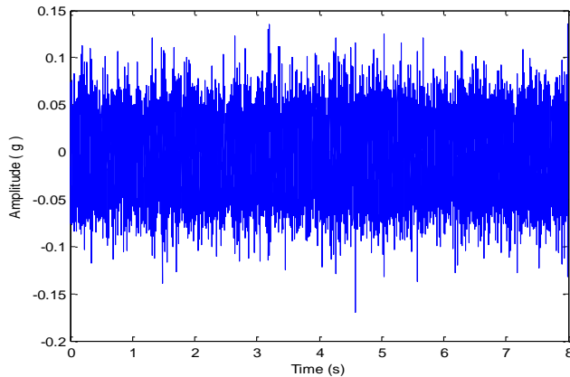
Gambar 9. Baseline 3000 rpm
