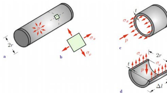
Gambar 1. Diagram benda bebas bejana tekan [3]
