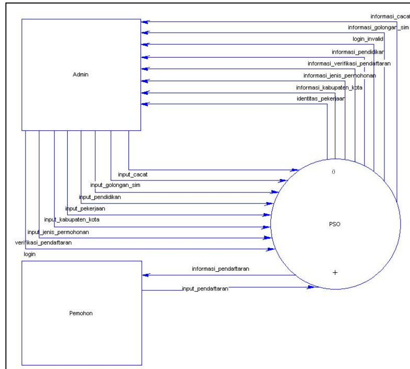
Gambar 5 Data Context Diagram (DCD)
