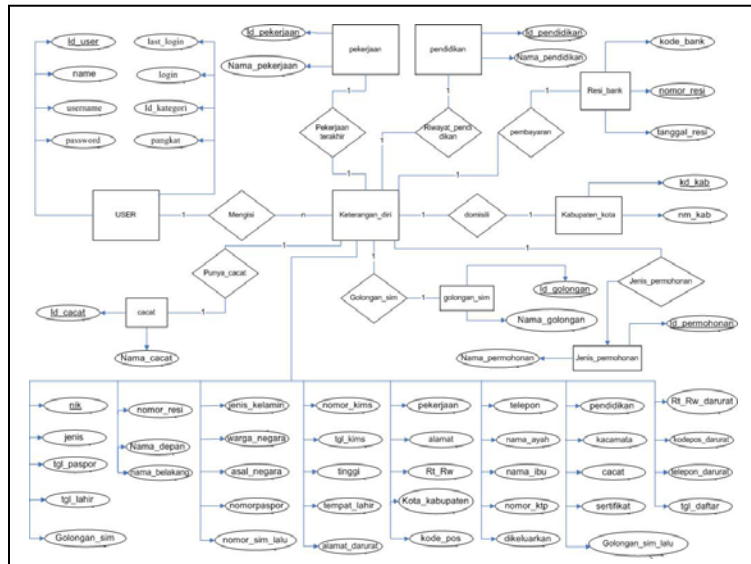
Gambar 4 Entity Relathionship Diagram
