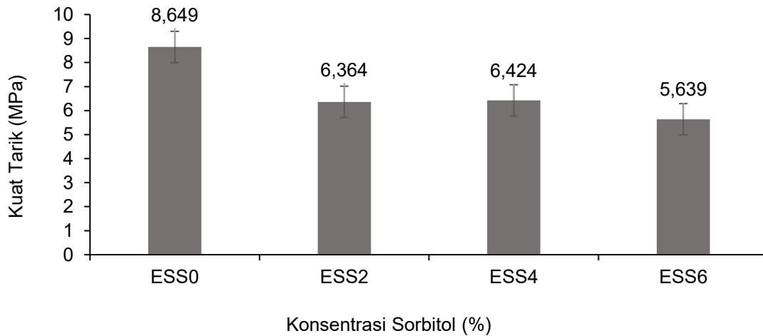
Gambar 2. Kuat tarik edible straw karagenan-sorbitol
