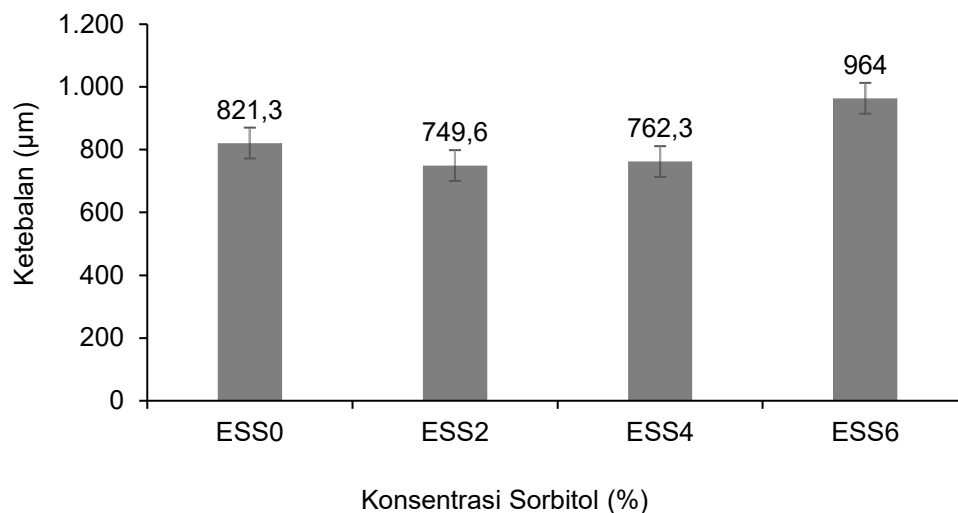
Gambar 4. Ketebalan edible straw karagenan-sorbitol
