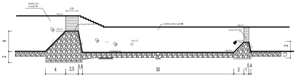
Gambar 4. Sketsa check dam
