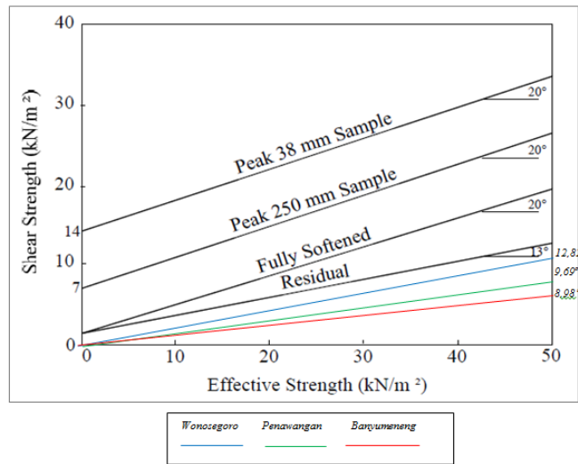
Gambar 7. Plot Hasil Pengujian Direct Shear (Sumber: Skempton, 1977)
