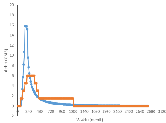
Gambar 9. Hidrograf Inflow dan Outflow Long Storage Tawang Sari
