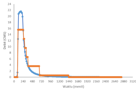
Gambar 7. Hidrograf Inflow dan Outflow Long Storage Semarang Indah
