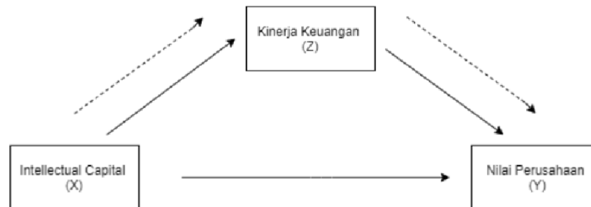
Gambar 1. Model Hipotesis
