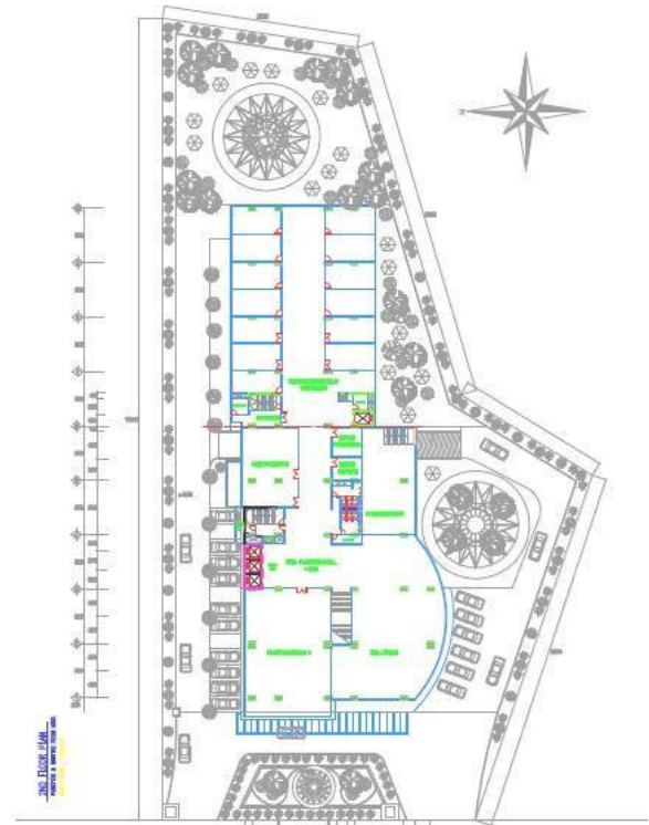
Denah Lantai 2
