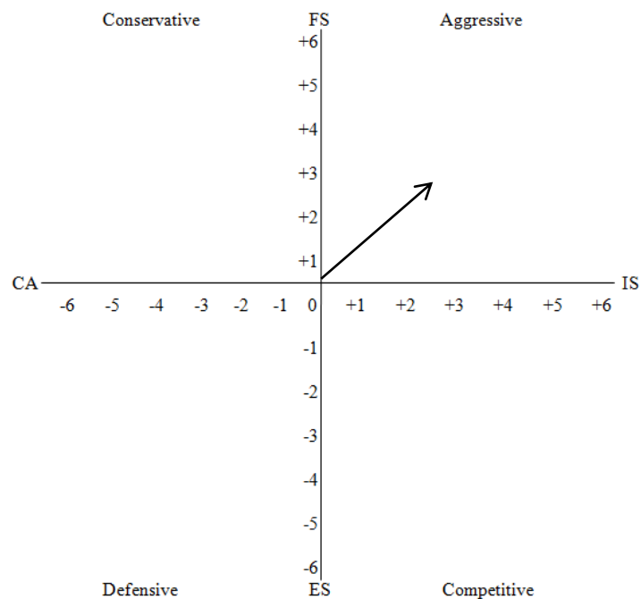
Gambar 2 Matriks SPACE
