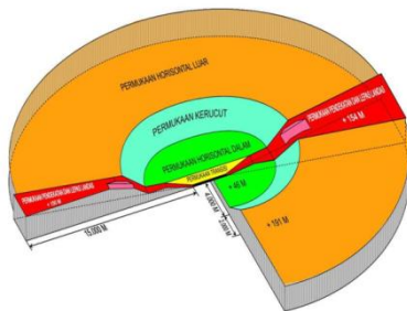
Gambar 2. Sketsa KKOP
