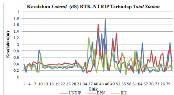
Gambar IV.4. Grafik kesalahan lateral (dS) RTK-NTRIP terhadap Total Station
