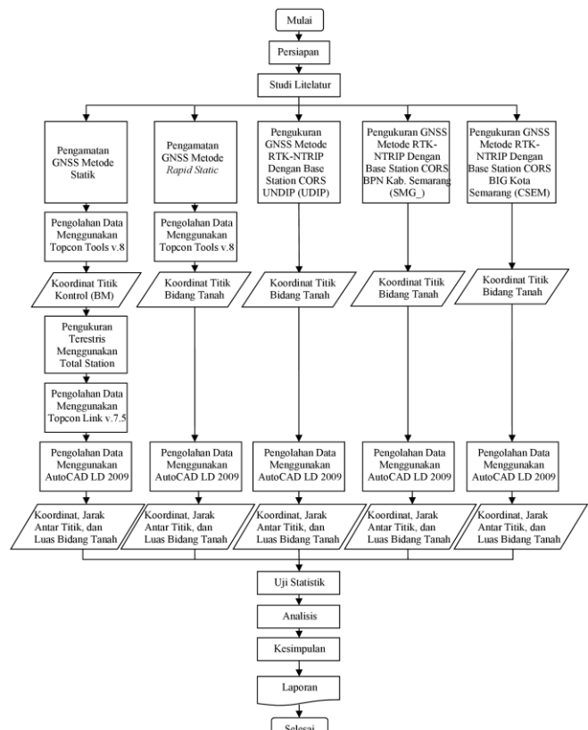
Gambar III.1. Diagram Alir Penelitian
