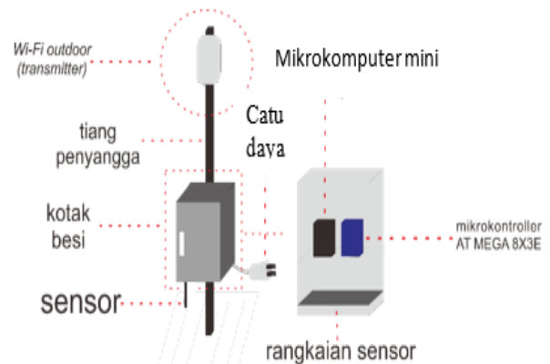
Gambar 3. Desain wireless sensor network
