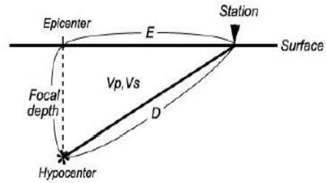
Gambar 4. Jarak hiposenter [7]
